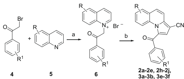
Scheme 1. Reagents and conditions: (a) \text{CH}_3\text{CN} , 85 °C, 4–6 h; (b) acrylonitrile, TPCD, DMF, \text{Na}_2\text{CO}_3 , 95 °C, 5 h or acrylonitrile, \text{MnO}_2 , DMF, \text{Et}_3\text{N} , 95 °C, 5 h.
