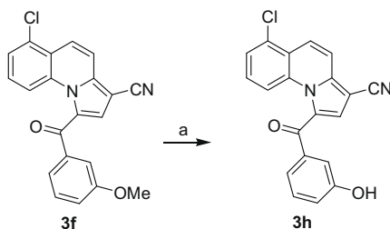
Scheme 5. Reagents and conditions: (a) \text{BBr}_3 , \text{CH}_2\text{Cl}_2 , –78 °C, then 10 °C, 1.5 h.
