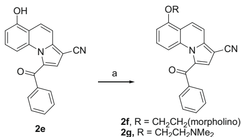
Scheme 2. Reagents and conditions: (a) \text{RCl} , acetone, \text{K}_2\text{CO}_3 , \text{KI} , 60 °C, 2.5 days.
