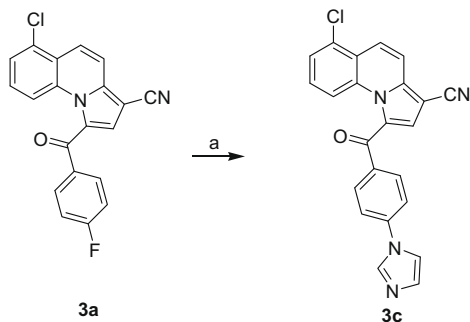
Scheme 3. Reagents and conditions: (a) imidazole, DMF, \text{K}_2\text{CO}_3 , 160 °C, 20 h.
