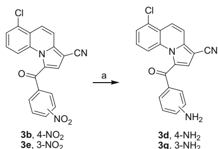
Scheme 4. Reagents and conditions: (a) \text{SnCl}_2 , \text{EtOH} , 90 °C, 7 h.
